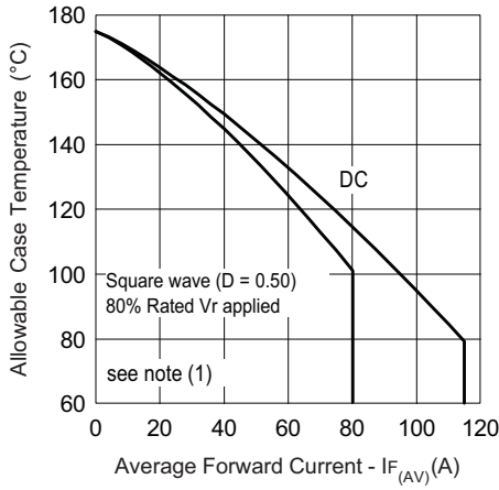
Fig. 2 - Maximum Allowable Case Temperature vs. Average Forward Current
