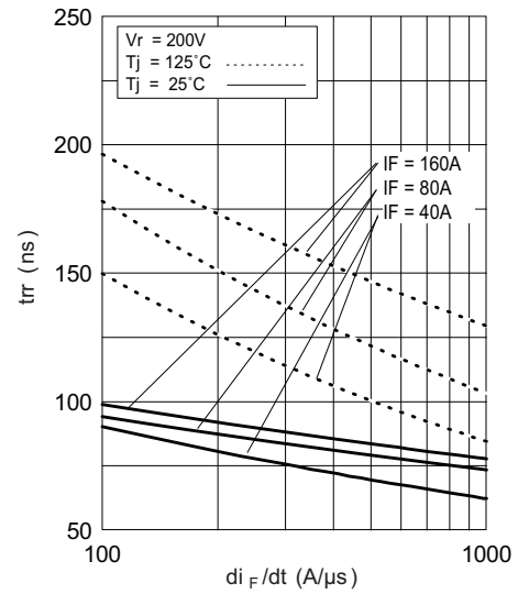
Fig. 5 - Typical Reverse Recovery Time vs. di_F/dt
