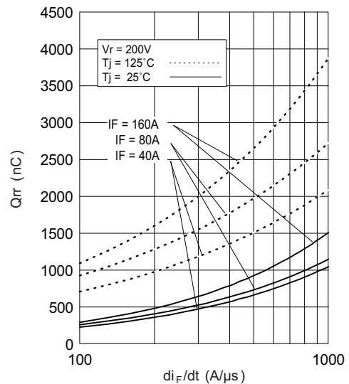
Fig. 6 - Typical Stored Charge vs. di_F/dt
